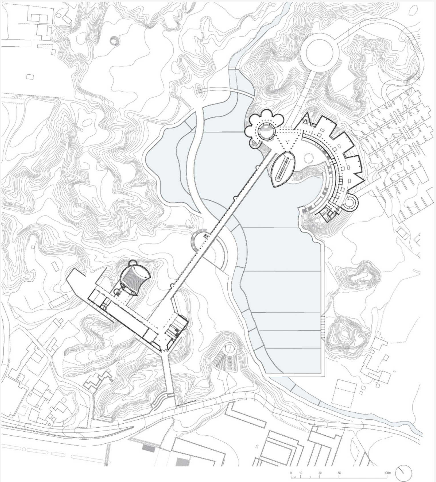
Khalsa Heritage Centre 7 Site plan
