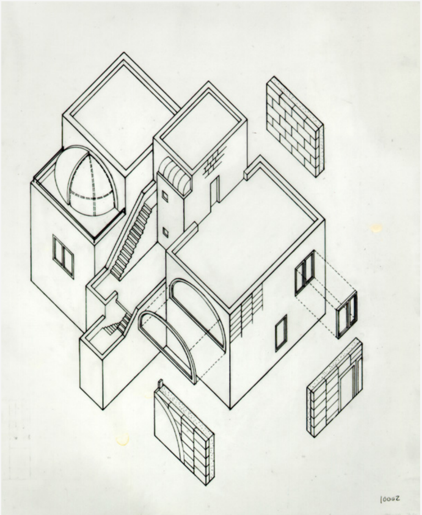
Block 38 Housing 3 Exploded axonometric
