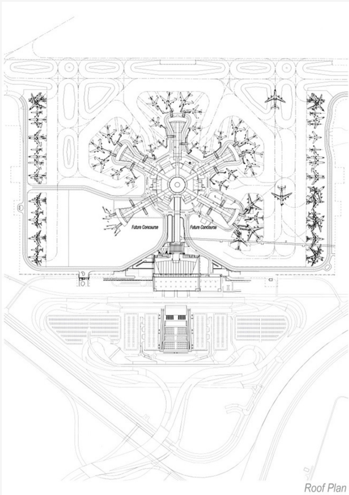
Ben Gurion Airport Airside Terminal 2 Site plan
