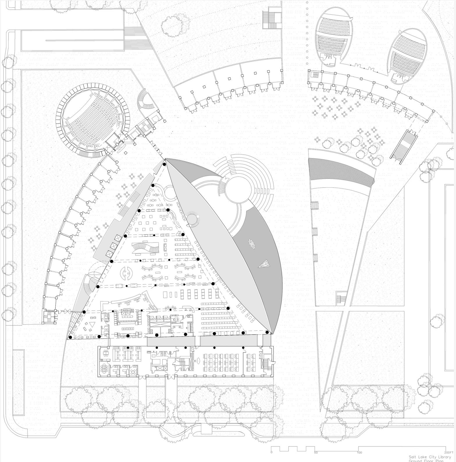
Salt Lake City Main Public Library 8 Entry level plan
